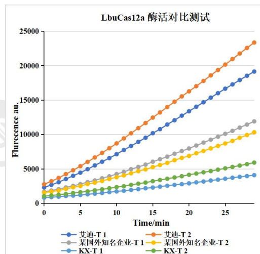
Fig 1. Results of Cas12a collateral cleavage at different company product.
